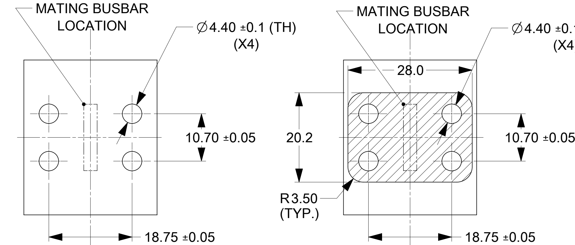
RECOMMENDED BUSBAR LAYOUT
