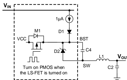
Figure 5: Internal Bootstrap Charging Circuit
