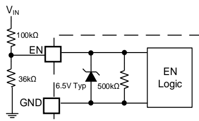
Figure 2: Zener Diode (6.5V Typical)
